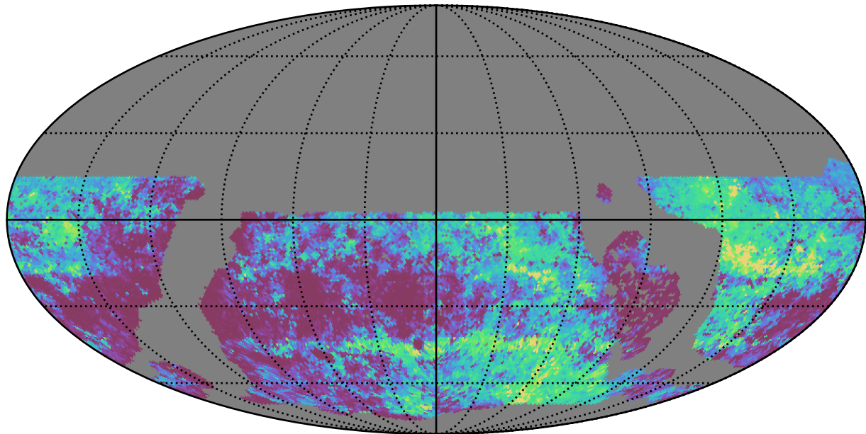
no_long_daily_v3.4_10yrs WFD ri bands: 75th Percentile Intranight Timespan
