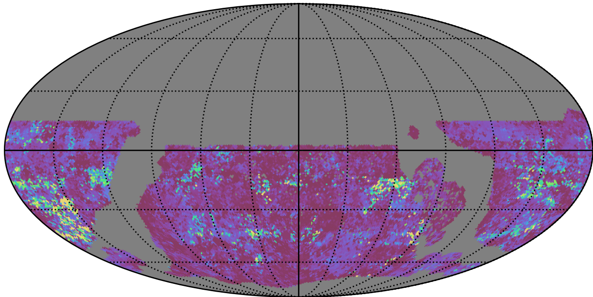
no_long_daily_v3.4_10yrs WFD g band: 75th Percentile Intranight Timespan
