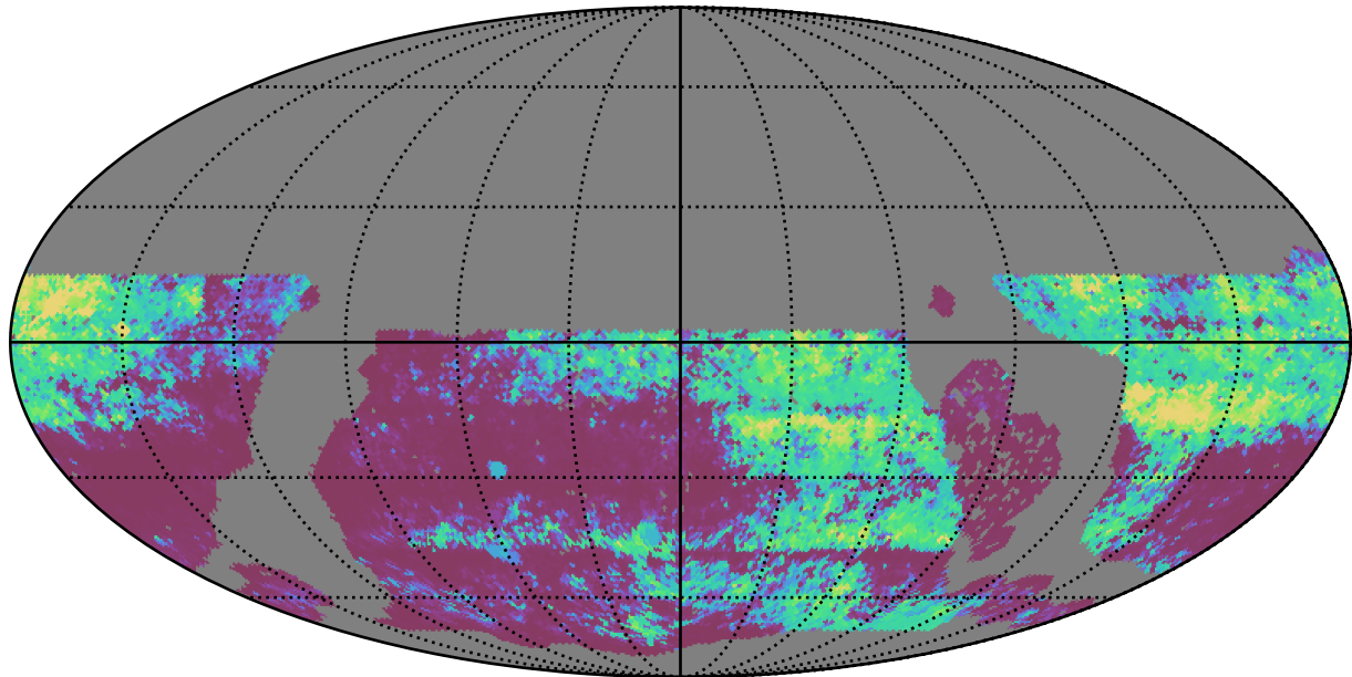
no_long_daily_v3.4_10yrs WFD all bands: 75th Percentile Intranight Timespan
