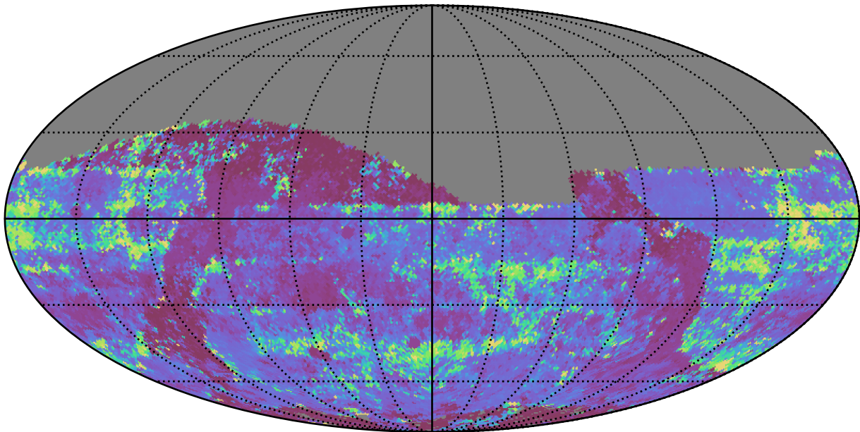
no_long_daily_v3.4_10yrs All sky z band: 75th Percentile Intranight Timespan
