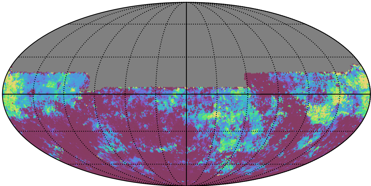
no_long_daily_v3.4_10yrs All sky y band: 75th Percentile Intranight Timespan
