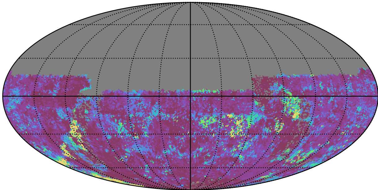
no_long_daily_v3.4_10yrs All sky u band: 75th Percentile Intranight Timespan
