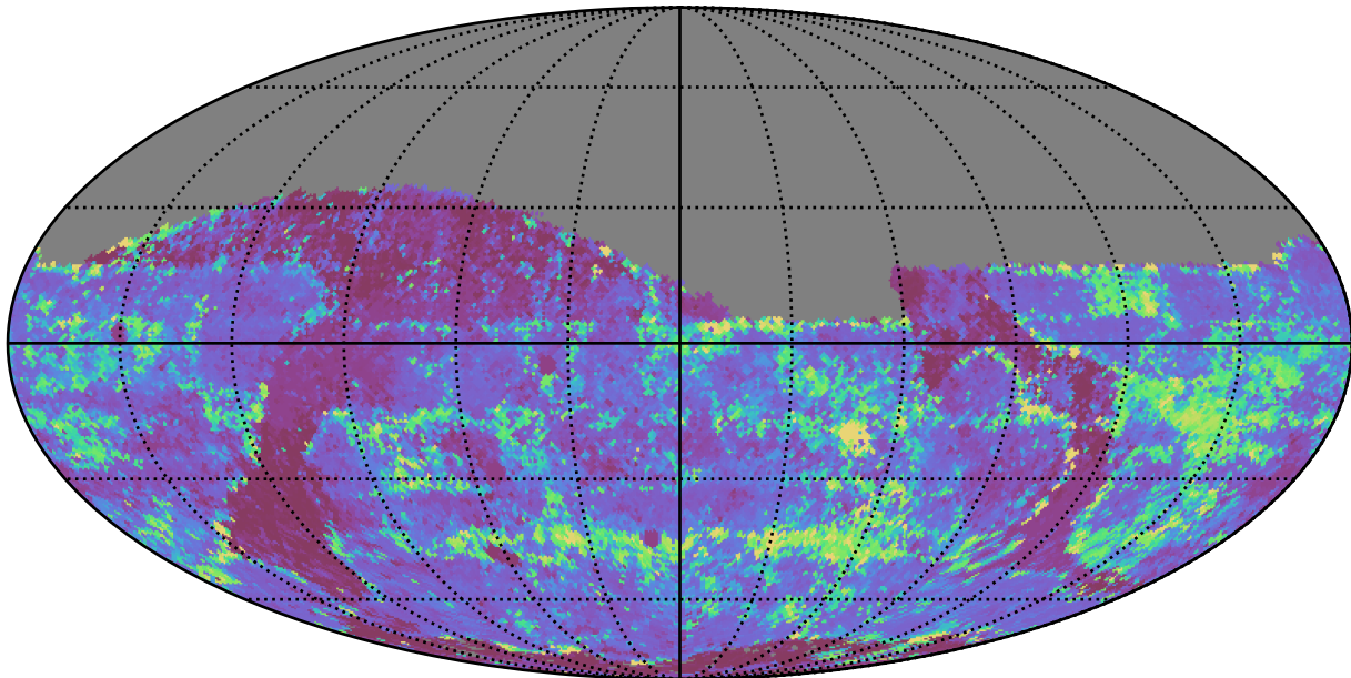
no_long_daily_v3.4_10yrs All sky r band: 75th Percentile Intranight Timespan
