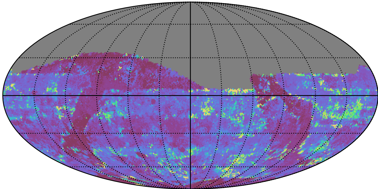
no_long_daily_v3.4_10yrs All sky i band: 75th Percentile Intranight Timespan
