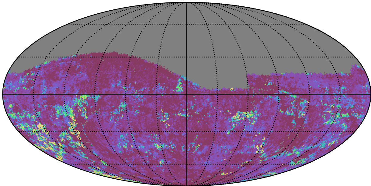
no_long_daily_v3.4_10yrs All sky g band: 75th Percentile Intranight Timespan
