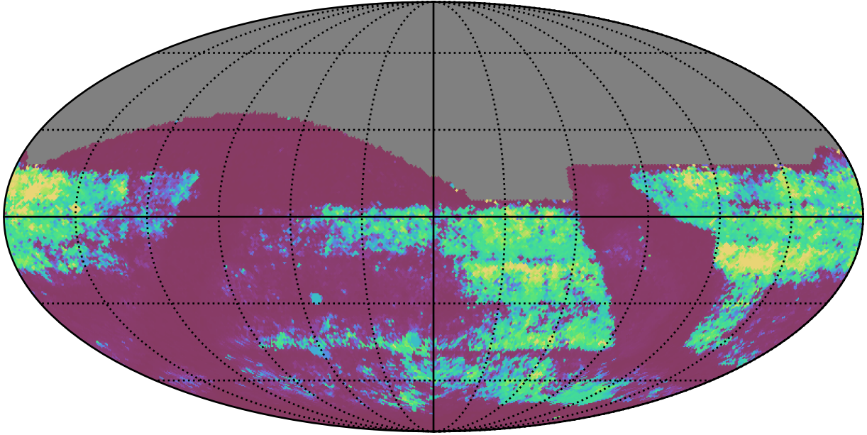
no_long_daily_v3.4_10yrs All sky all bands: 75th Percentile Intranight Timespan
