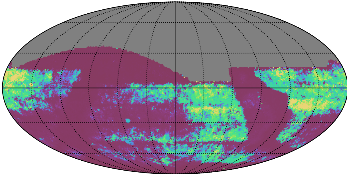
no_long_daily_v3.4_10yrs All sky: 75th Percentile Intranight Timespan
