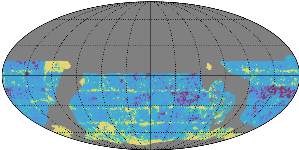
no_long_daily_v3.4_10yrs WFD r band: 20thPercentile Inter-Night Gap
