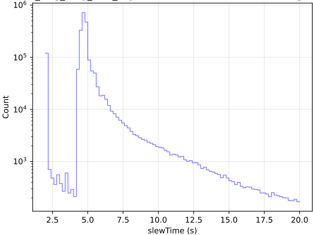
no_long_daily_v3.4_10yrs All visits: Zoom Slew Time Histogram
