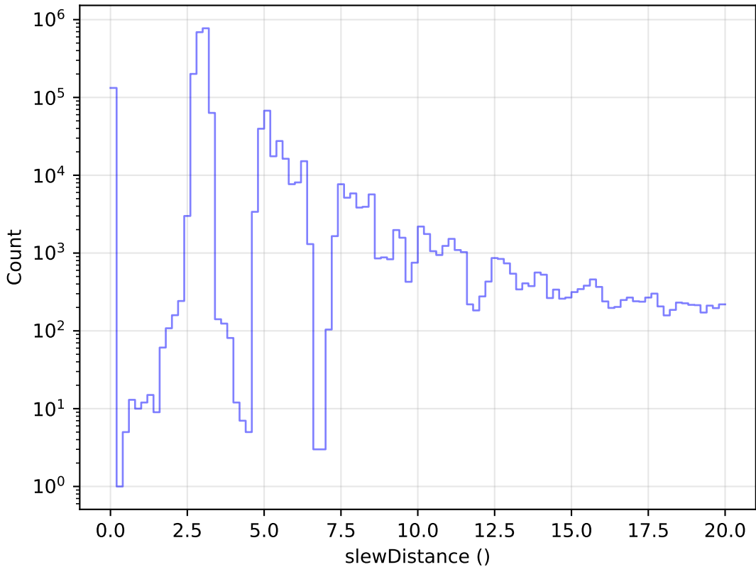
no_long_daily_v3.4_10yrs All visits: Zoom Slew Distance Histogram
