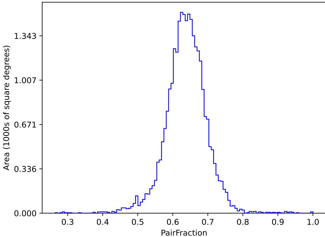
no_long_daily_v3.4_10yrs (g or r or i): PairFraction
