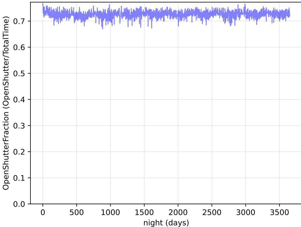
no_long_daily_v3.4_10yrs : OpenShutterFraction
