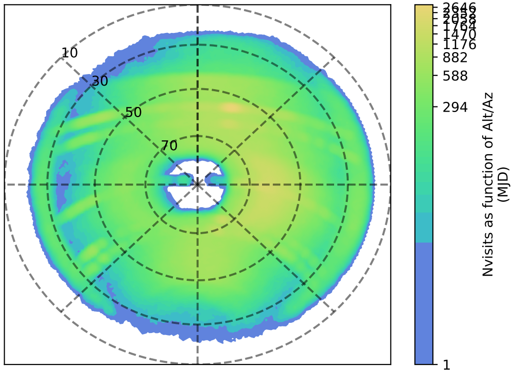
no_long_daily_v3.4_10yrs z: Nvisits as function of Alt/Az
