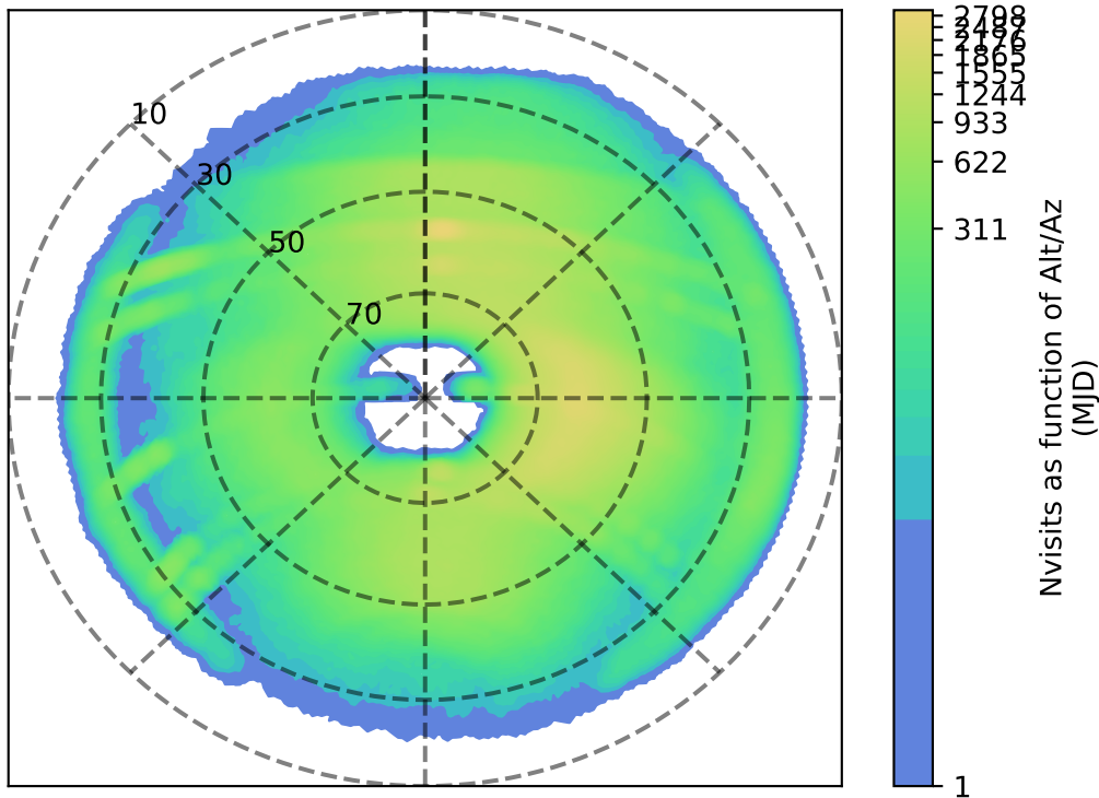
no_long_daily_v3.4_10yrs i: Nvisits as function of Alt/Az
