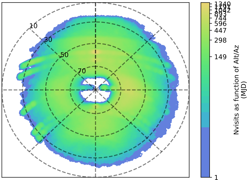
no_long_daily_v3.4_10yrs g: Nvisits as function of Alt/Az
