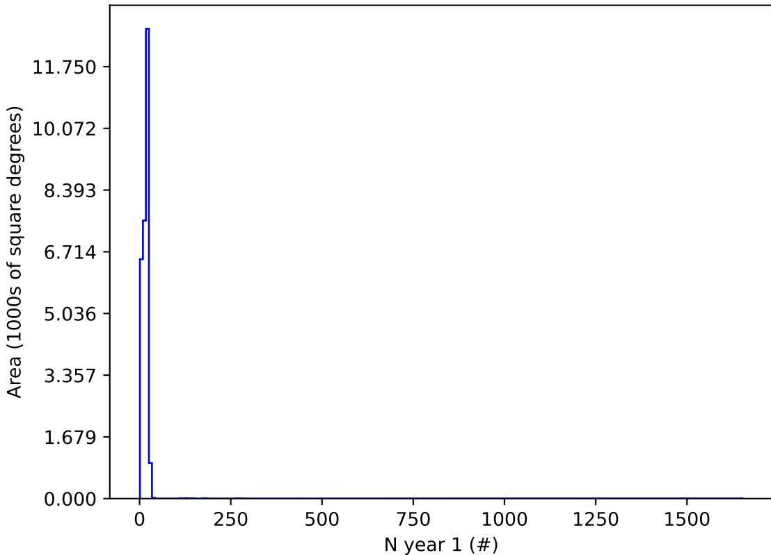
no_long_daily_v3.4_10yrs r and night < 365: N year 1
