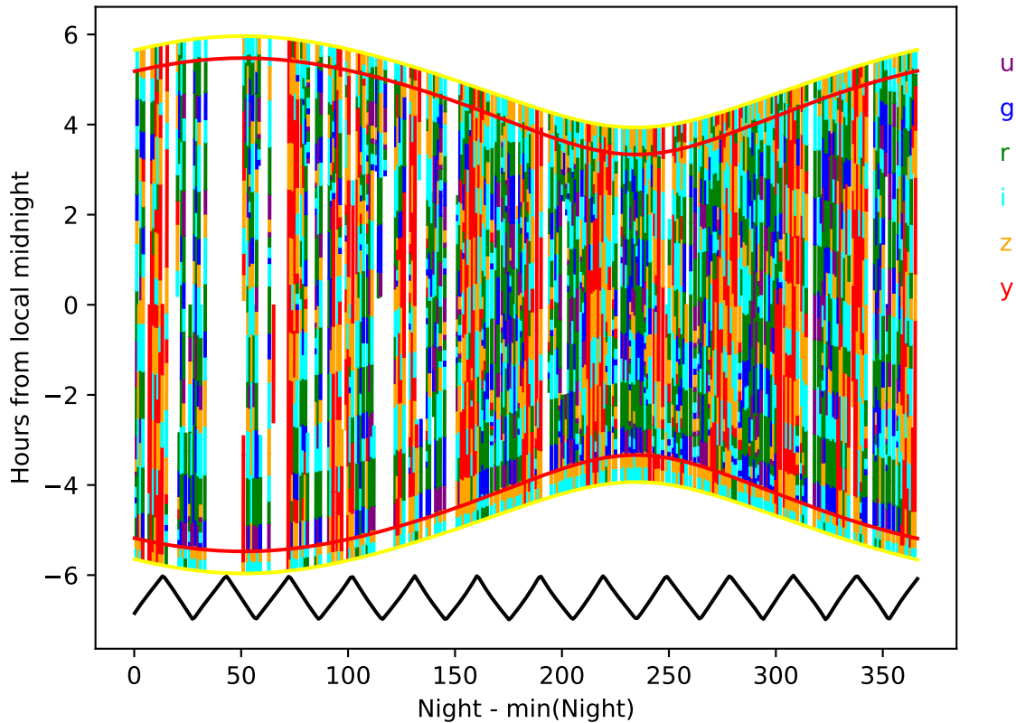
no_long_daily_v3.4_10yrs year 8-9: Hourglass
