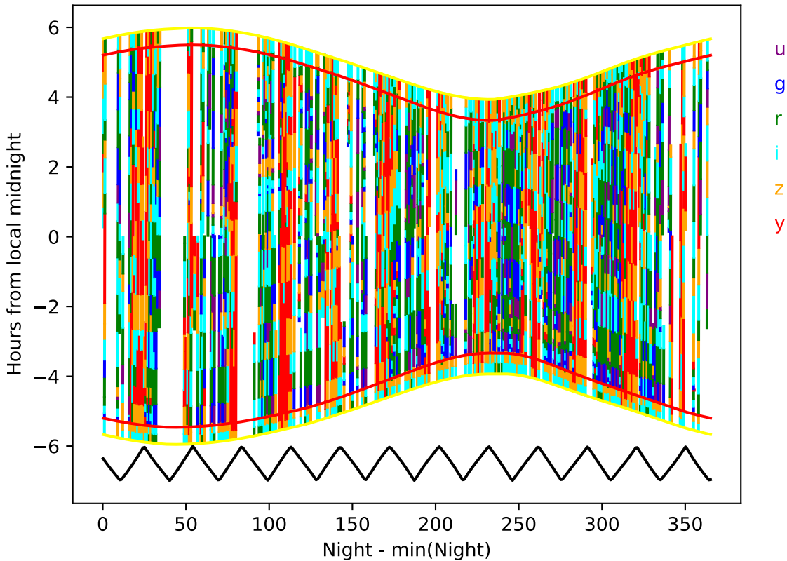
no_long_daily_v3.4_10yrs year 4-5: Hourglass
