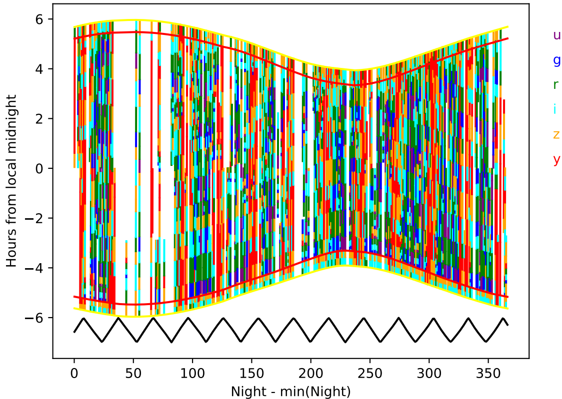
no_long_daily_v3.4_10yrs year 3-4: Hourglass
