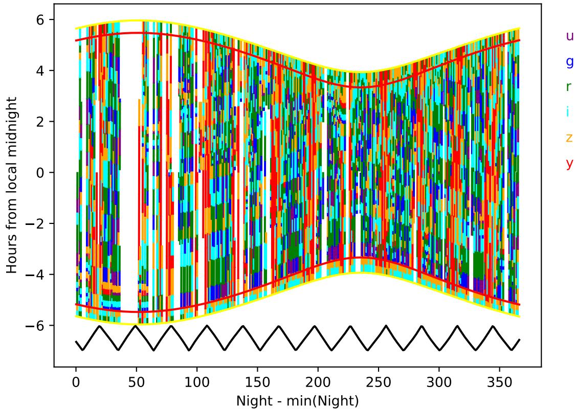
no_long_daily_v3.4_10yrs year 2-3: Hourglass
