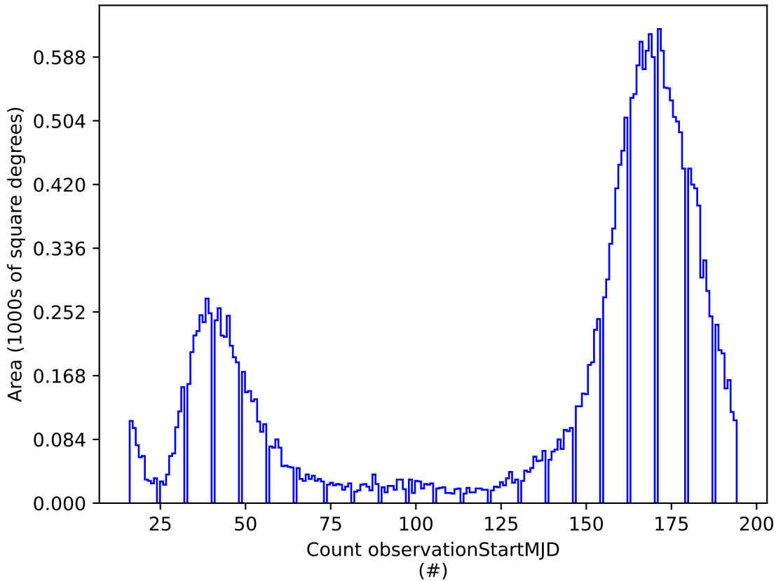
no_long_daily_v3.4_10yrs z: Count observationStartMJD
