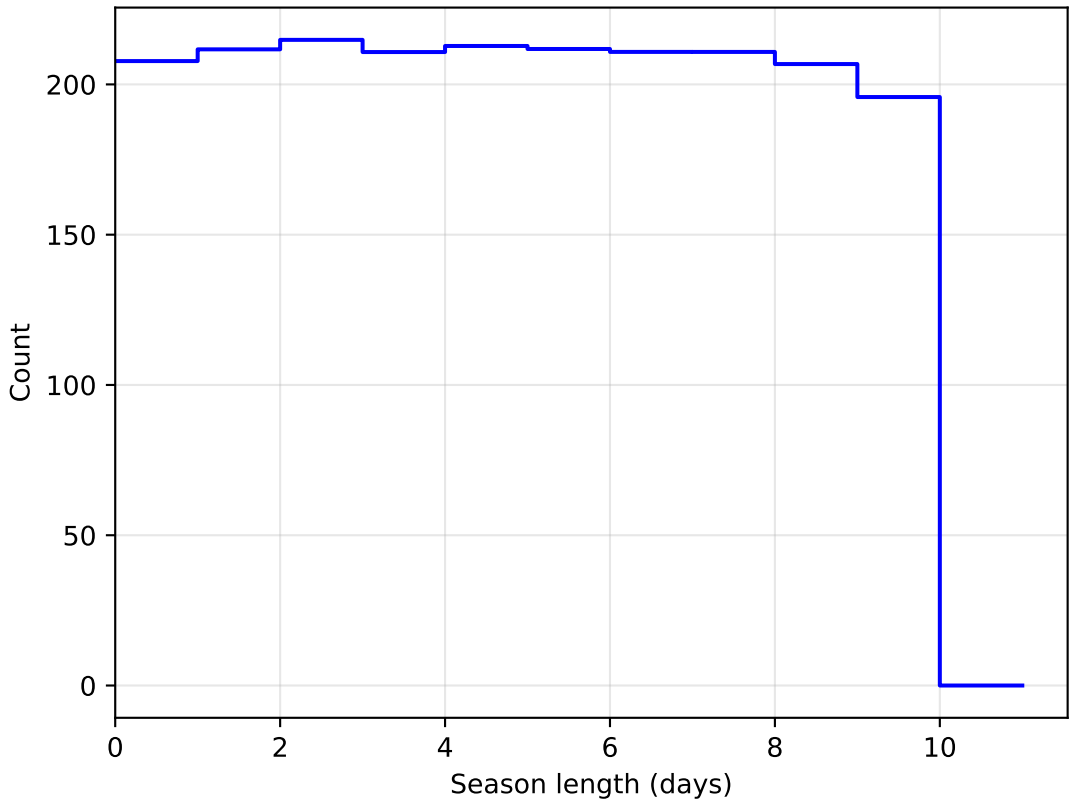
no_long_daily_v3.4_10yrs DD:EDFS all bands: SeasonLength
