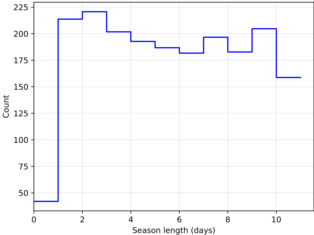
no_long_daily_v3.4_10yrs DD: COSMOS all bands: SeasonLength
