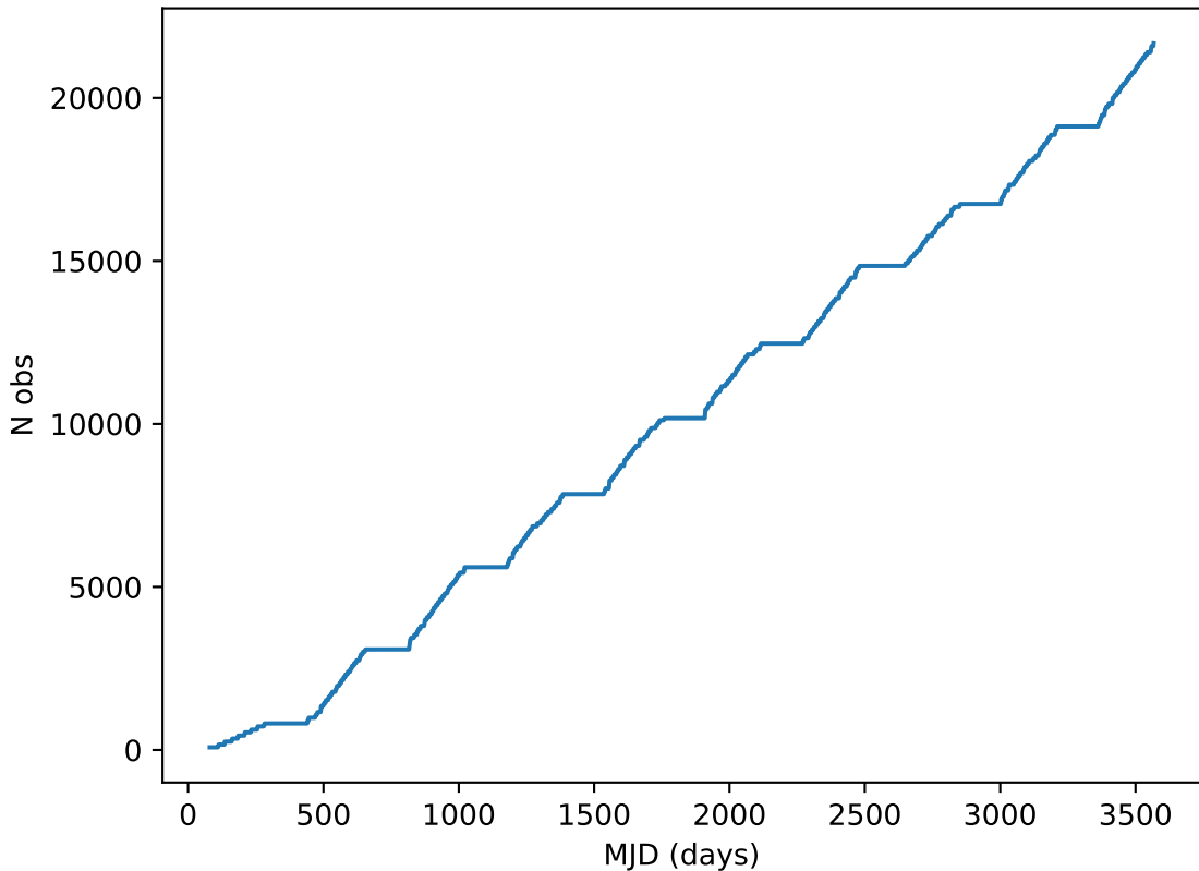
no_long_daily_v3.4_10yrs all bands: DD:XMM_LSS Cumulative NVisits
