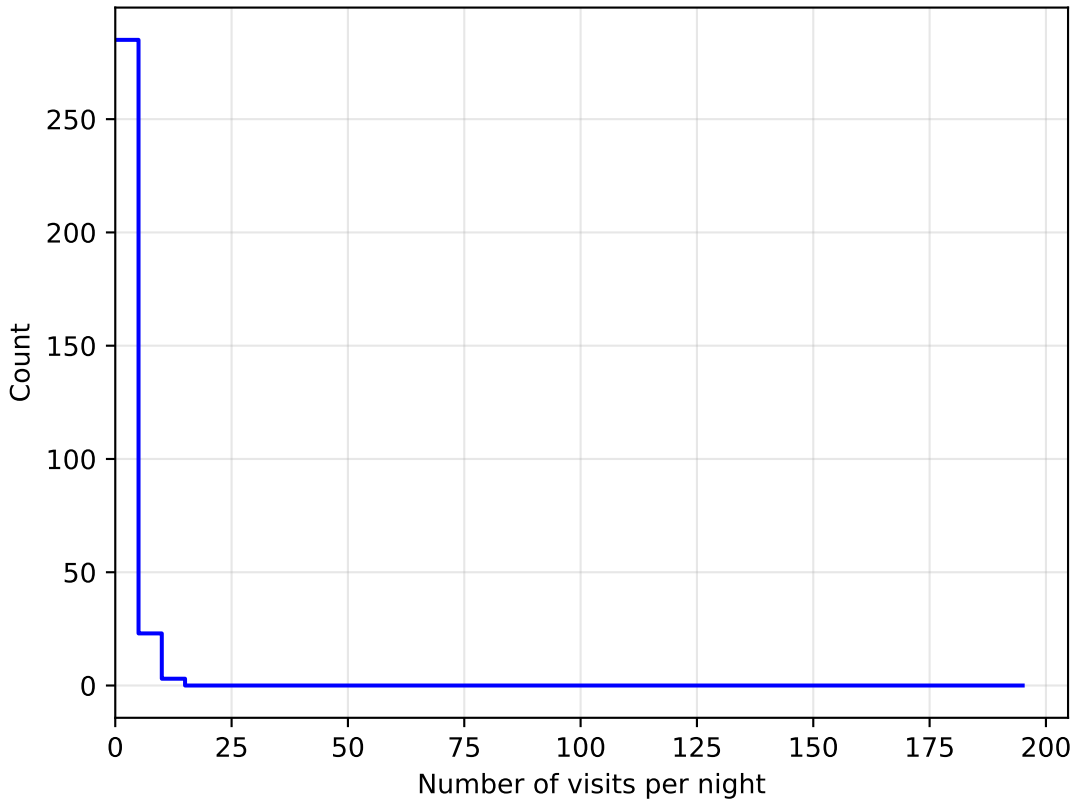
no_long_daily_v3.4_10yrs all bands: DD:WFD NVisitsPerNight
