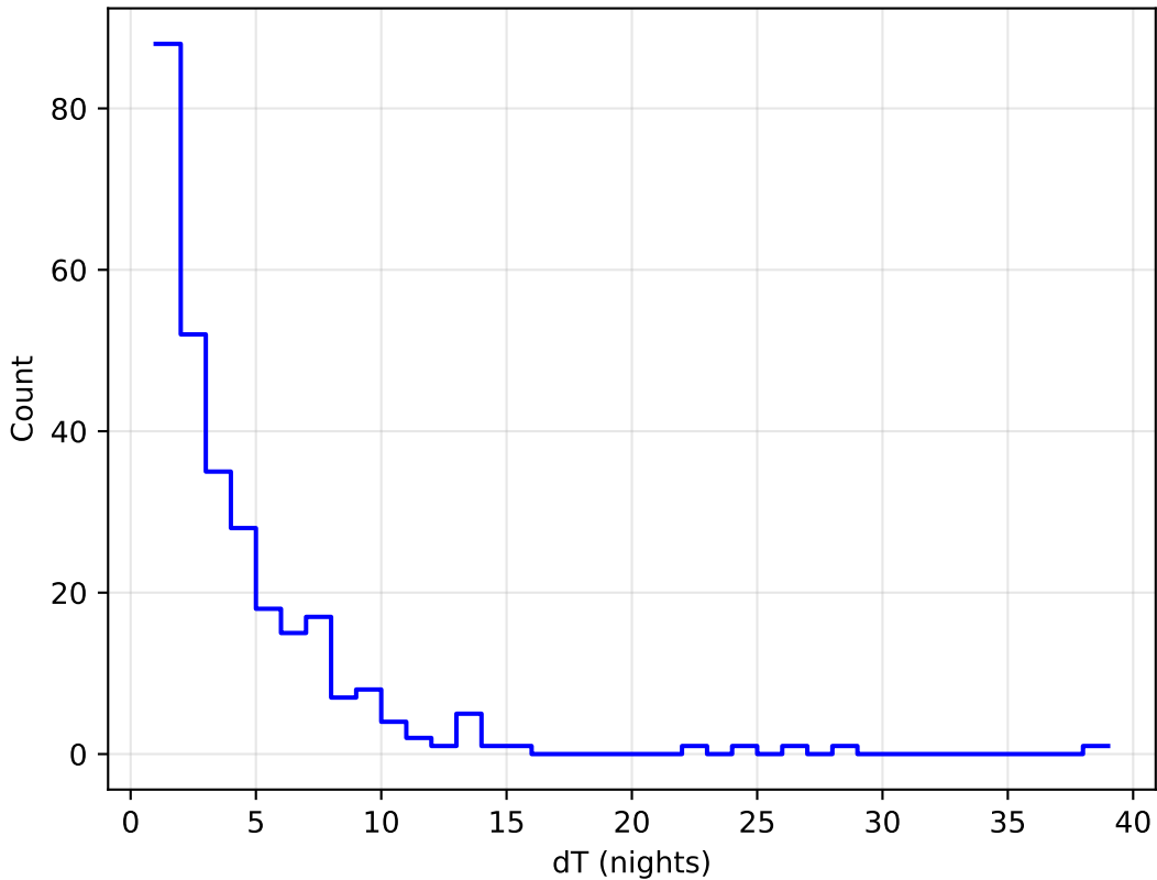
no_long_daily_v3.4_10yrs all bands: DD:WFD Delta Nights Histogram
