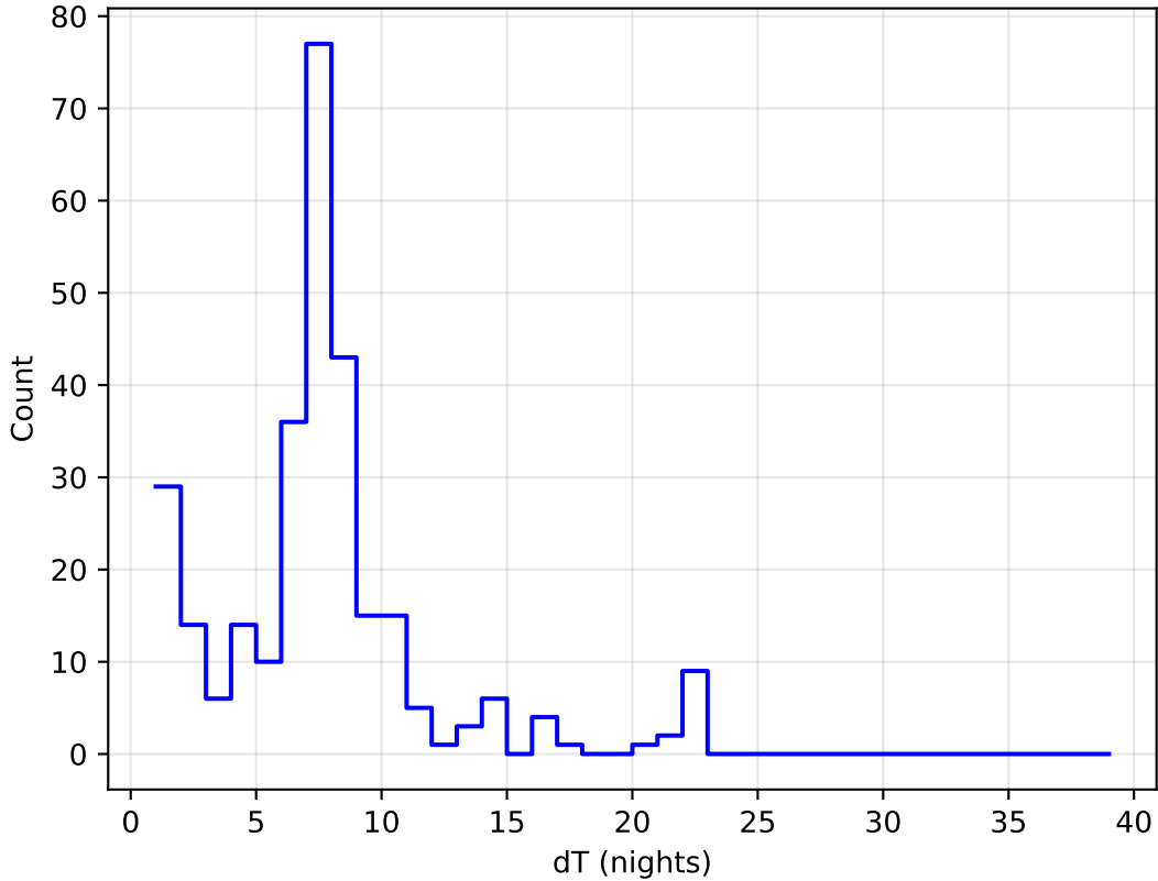
no_long_daily_v3.4_10yrs all bands: DD:EDFS Delta Nights Histogram
