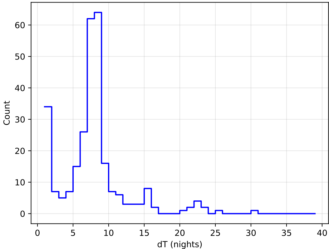
no_long_daily_v3.4_10yrs all bands: DD:ECDFS Delta Nights Histogram
