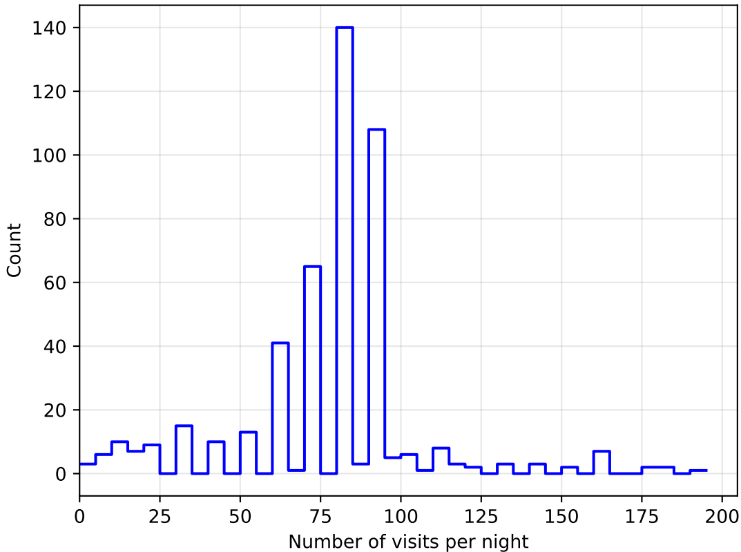
no_long_daily_v3.4_10yrs all bands: DD: COSMOS NVisitsPerNight
