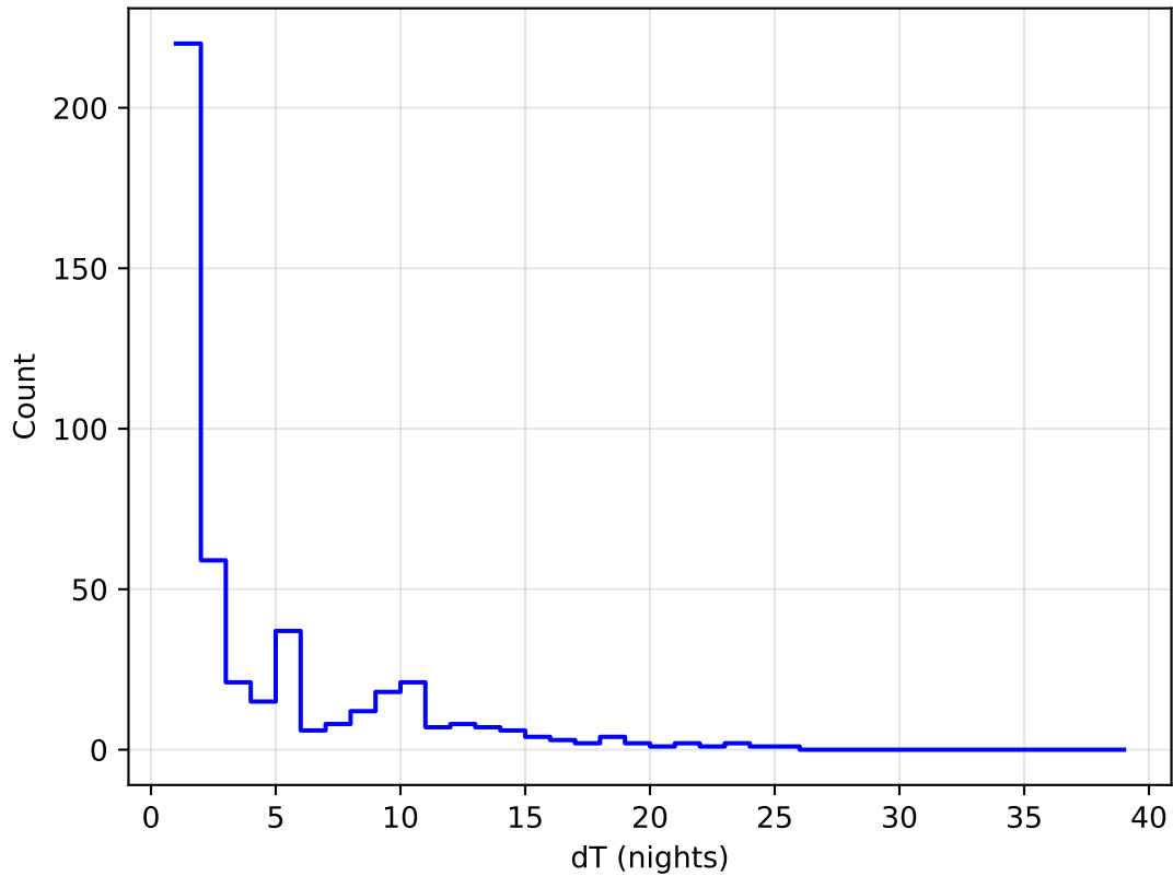
no_long_daily_v3.4_10yrs all bands: DD: COSMOS Delta Nights Histogram
