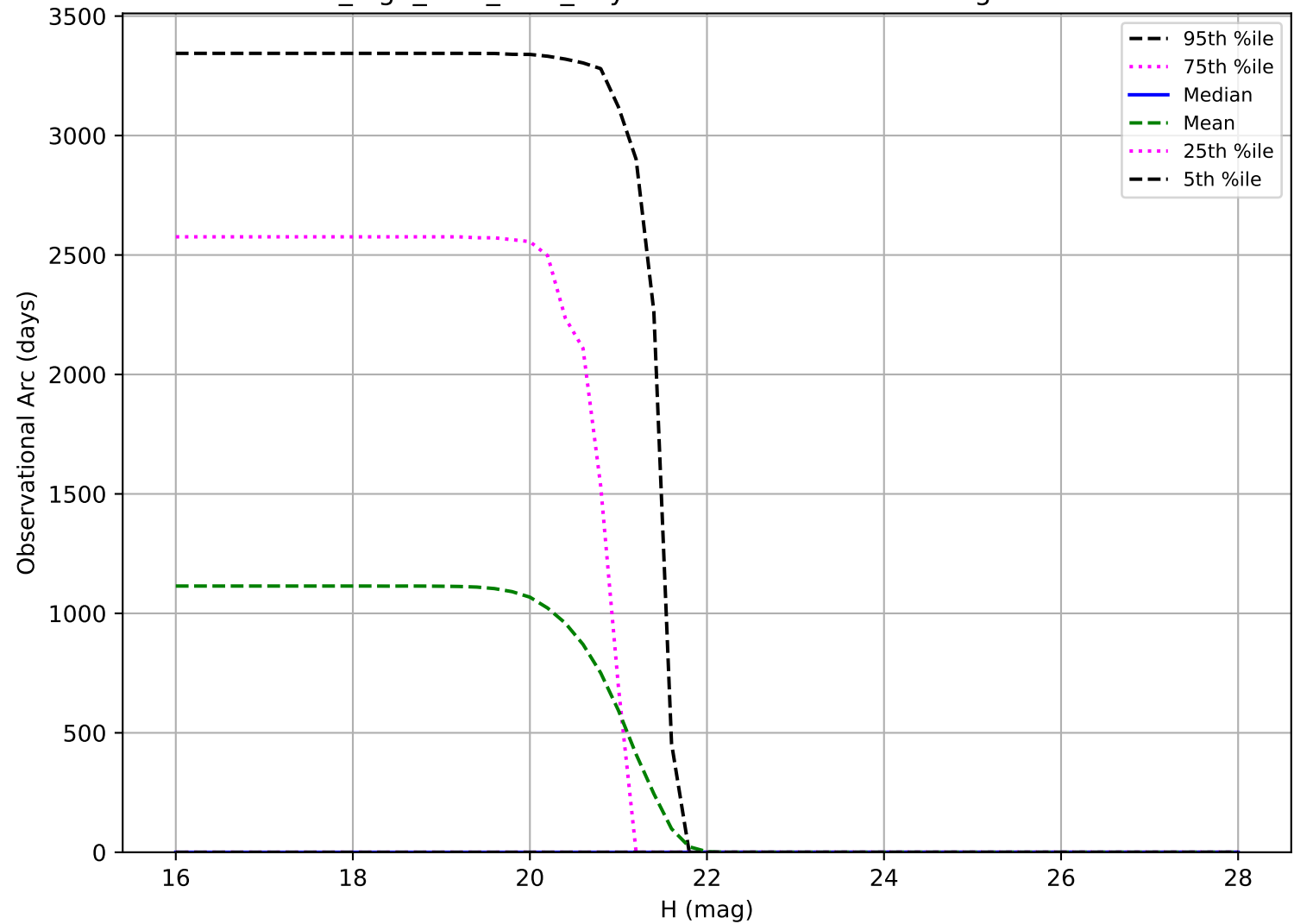
no_high_blob_v3.3_10yrs: Observational Arc Length Vatira
