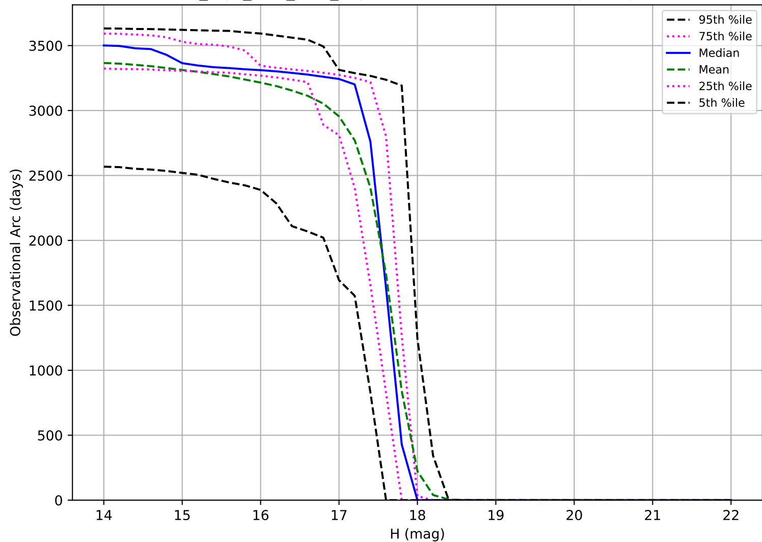
no_high_blob_v3.3_10yrs: Observational Arc Length Trojan
