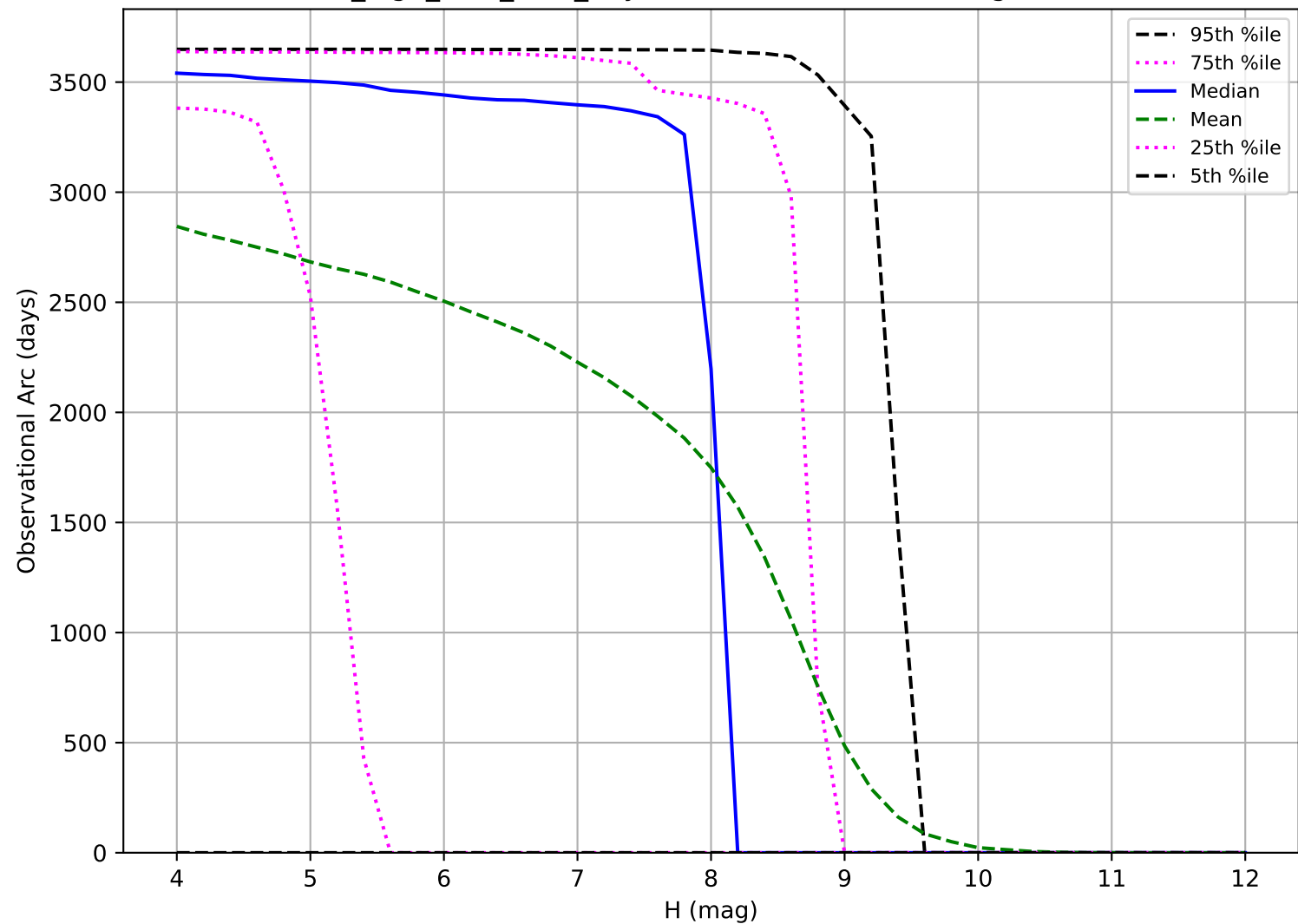
no_high_blob_v3.3_10yrs: Observational Arc Length TNO
