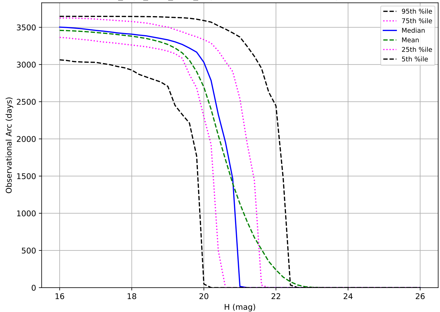
no_high_blob_v3.3_10yrs: Observational Arc Length MBA
