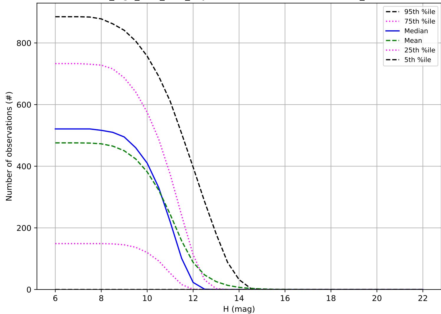
no_high_blob_v3.3_10yrs: Number of observations OCC_r20
