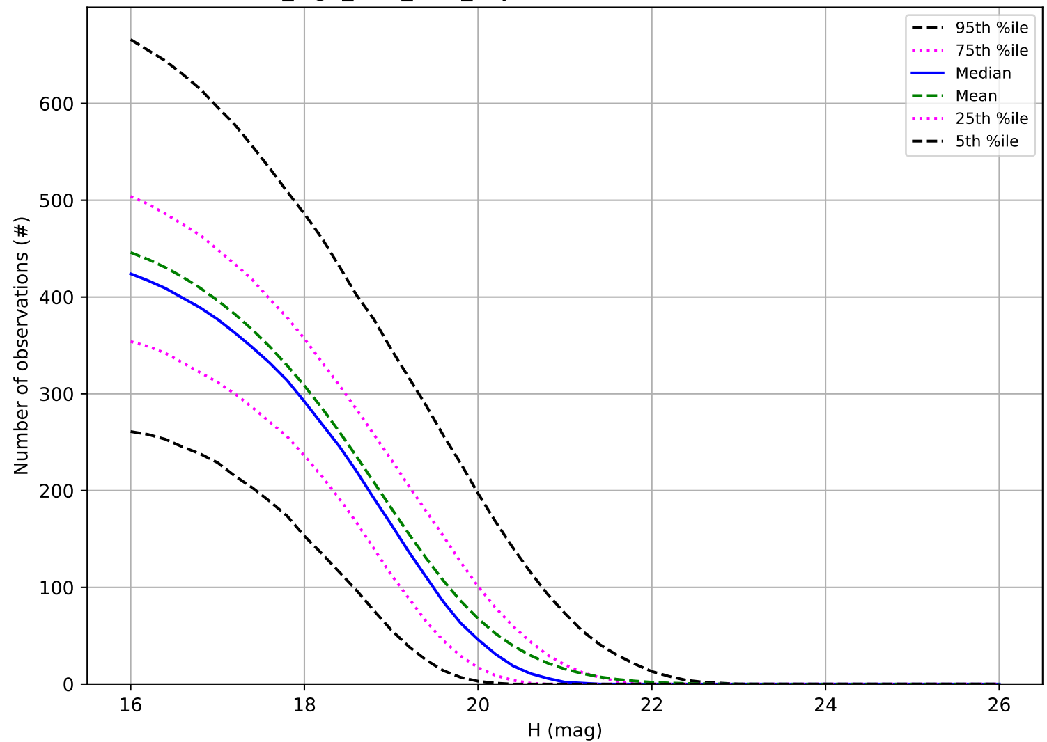
no_high_blob_v3.3_10yrs: Number of observations MBA
