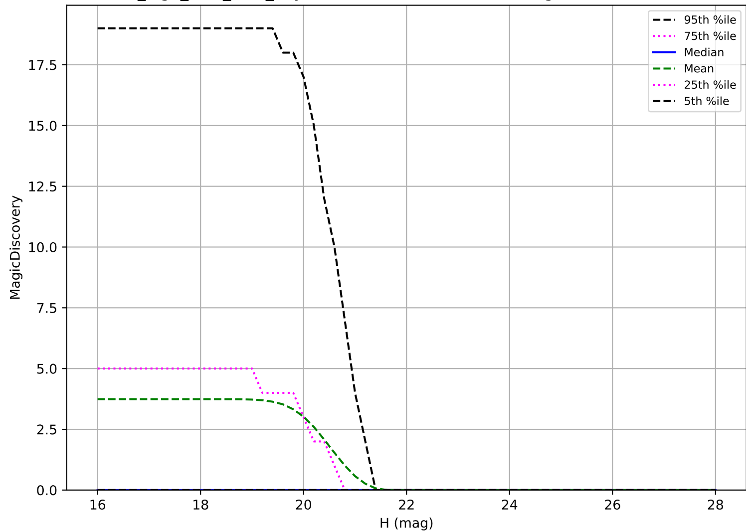
no_high_blob_v3.3_10yrs: Vatira 6 detections in 60 nights detection loss
