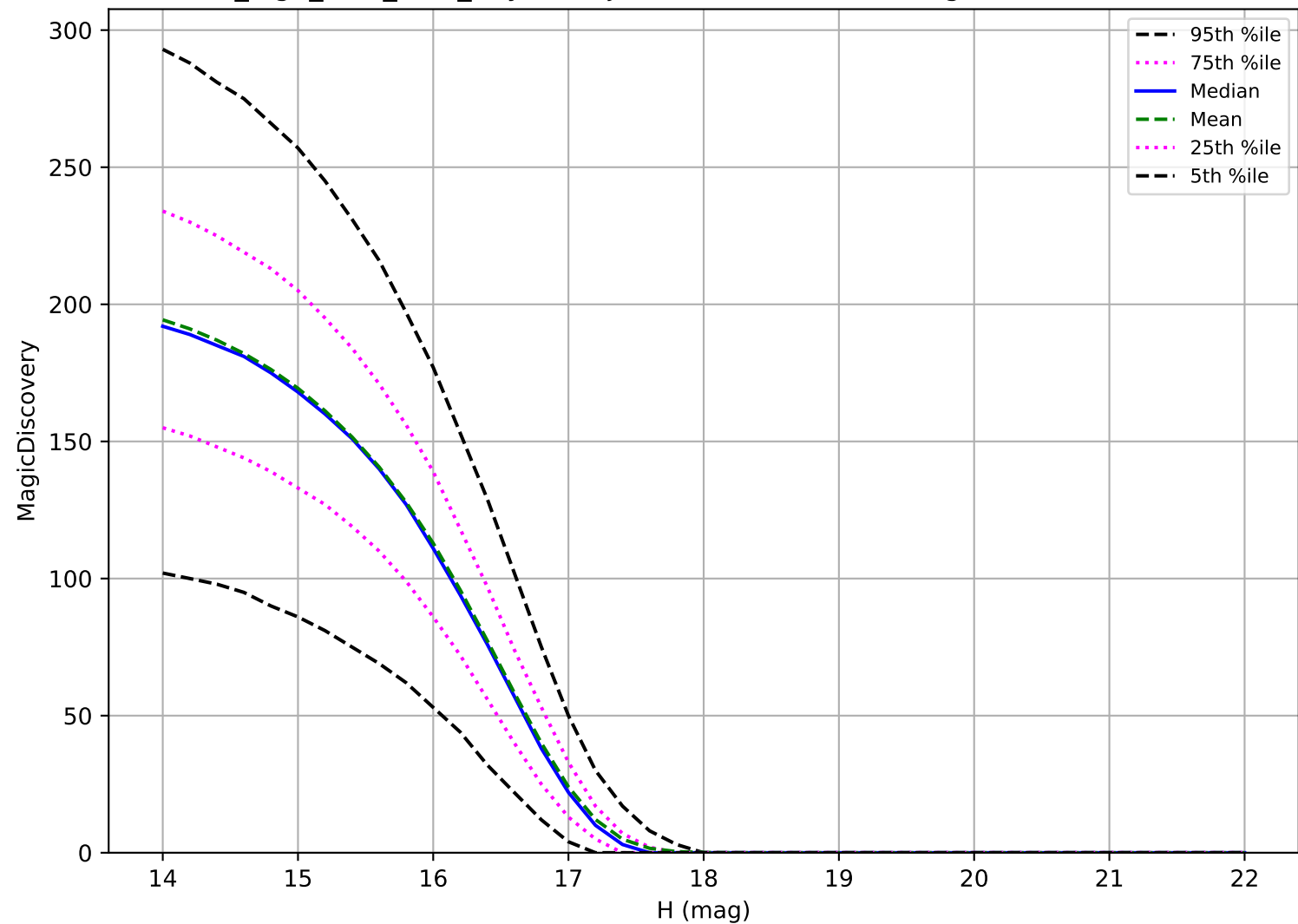
no_high_blob_v3.3_10yrs: Trojan 6 detections in 60 nights detection loss
