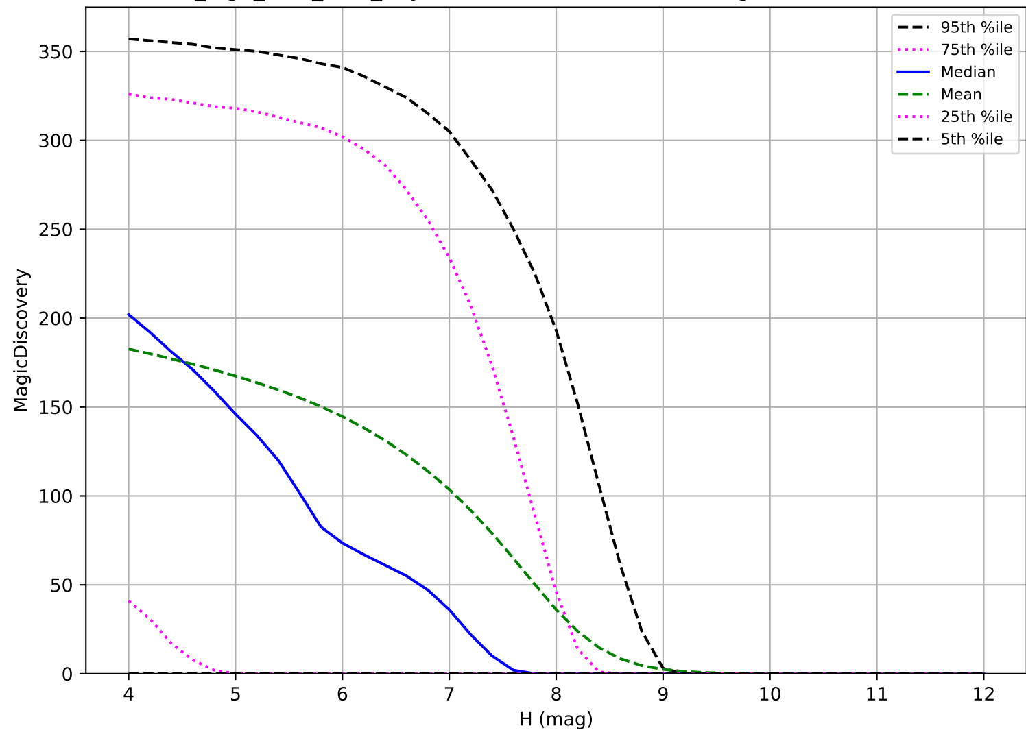
no_high_blob_v3.3_10yrs: TNO 6 detections in 60 nights detection loss
