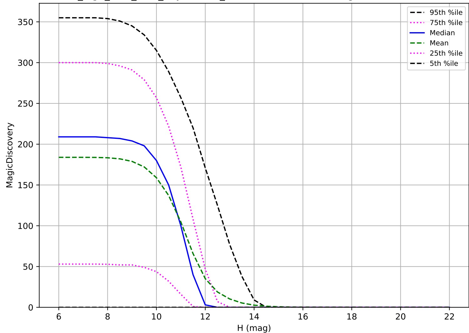
no_high_blob_v3.3_10yrs: OCC_r20 6 detections in 60 nights detection loss
