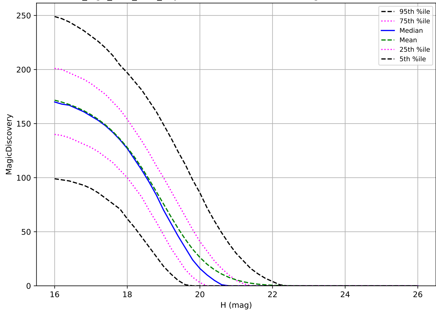
no_high_blob_v3.3_10yrs: MBA 6 detections in 60 nights detection loss
