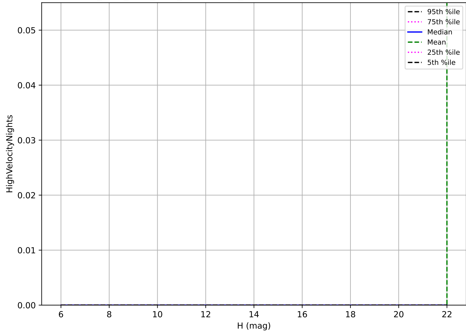
no_high_blob_v3.3_10yrs: OCC_r20 High velocity pair detection loss
