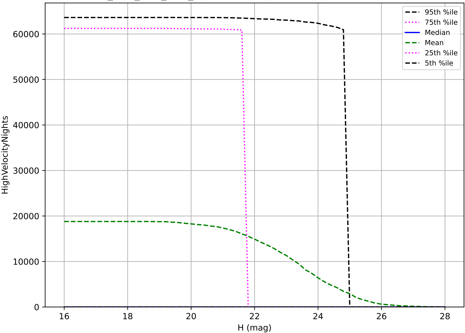
no_high_blob_v3.3_10yrs: NEO High velocity pair detection loss
