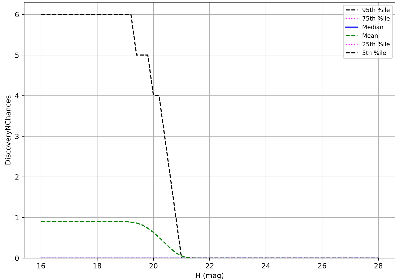
no_high_blob_v3.3_10yrs: Vatira 3 pairs in 15 nights detection loss
