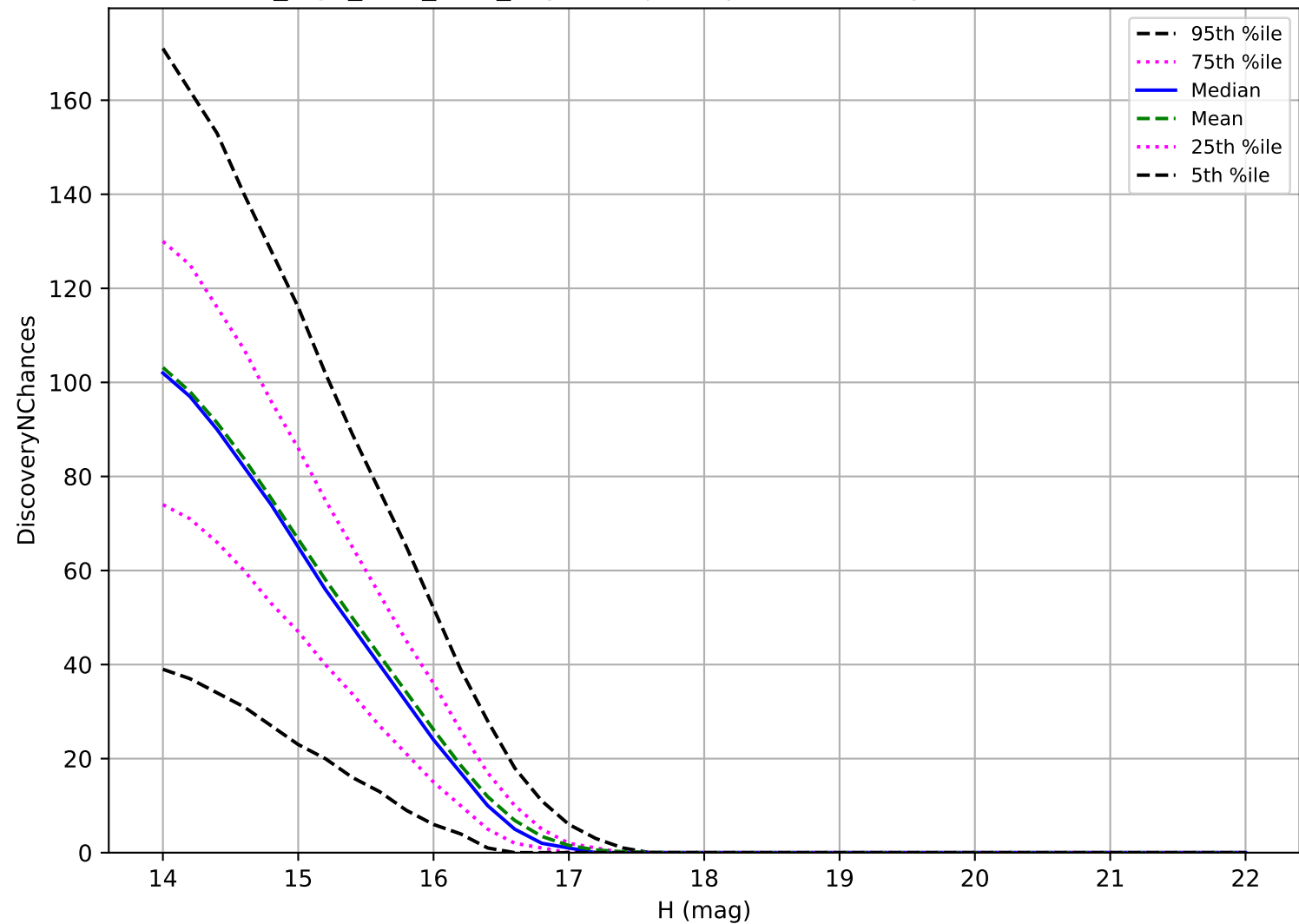
no_high_blob_v3.3_10yrs: Trojan 3 pairs in 15 nights detection loss
