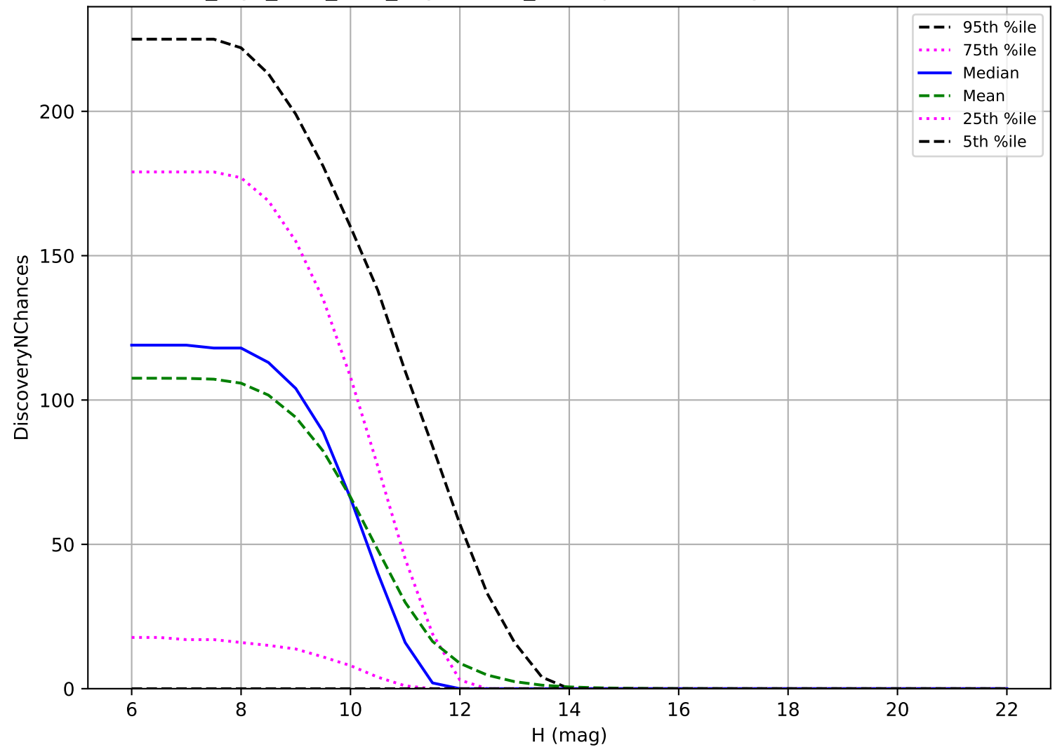
no_high_blob_v3.3_10yrs: OCC_r20 3 pairs in 15 nights detection loss
